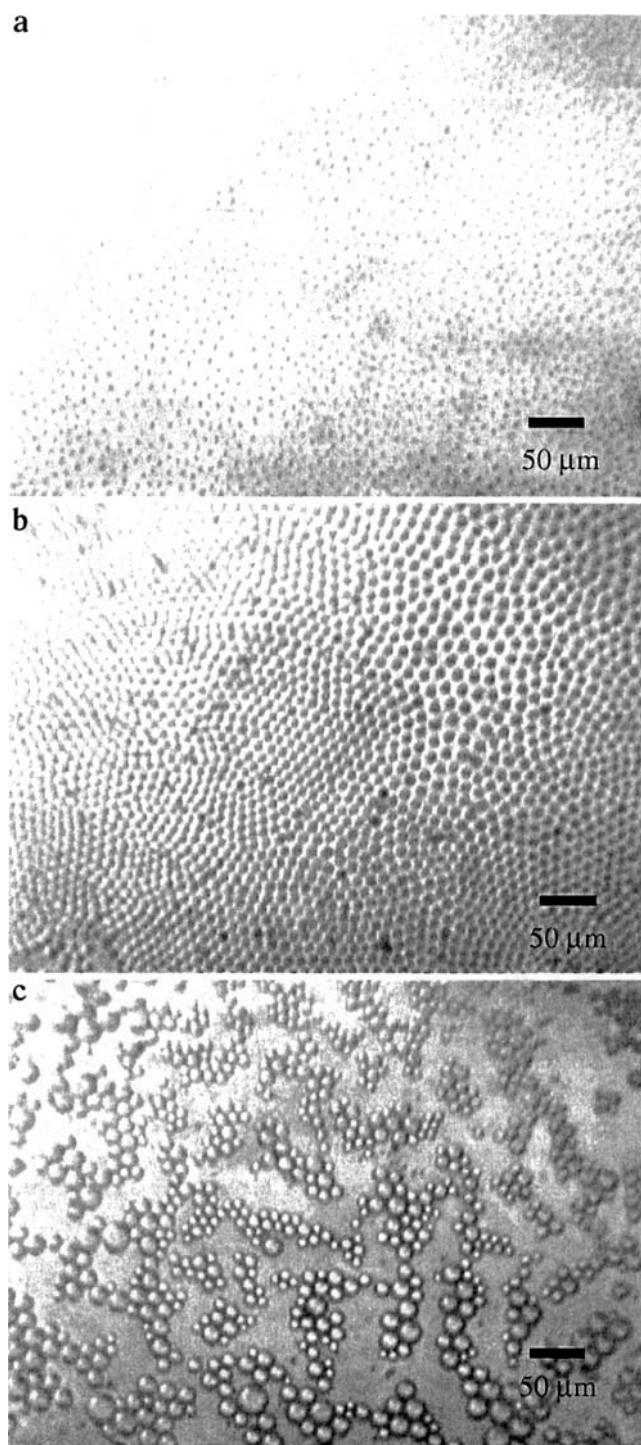
Fig. 3 Optical microscopy images of the self-assembling pattern for the colloidal suspension with a concentration of 0.12 wt% ZrO_2 and 2.0 wt% PVME at a 1,466, b 1,858, and c 2,046 s
