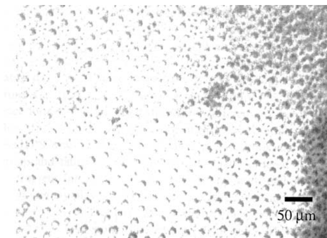
Fig. 4 Optical microscopy image for the colloidal suspension with a concentration of 0.12 wt% ZrO_2 and 1.0 wt% PVME at 1,258 s
