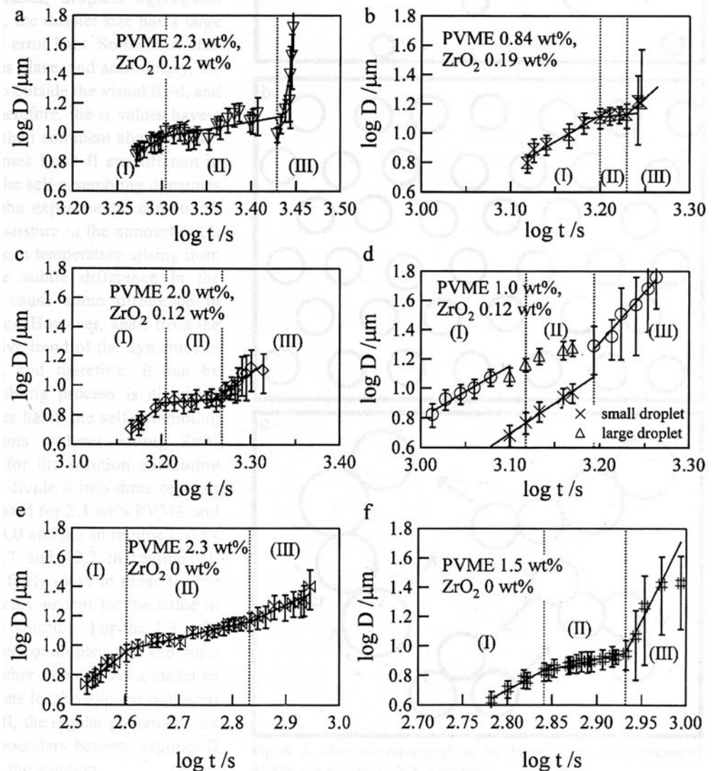
Fig. 7 Time change in the droplet size for various samples: a 0.12 wt% ZrO_2 and 2.3 wt% PVME, b 0.19 wt% ZrO_2 and 0.84 wt% PVME, c 0.12 wt% ZrO_2 and 2.0 wt% PVME, d 0.12 wt% ZrO_2 and 1.0 wt% PVME, e 0 wt% ZrO_2 and 2.3 wt% PVME, f 0 wt% ZrO_2 and 1.5 wt% PVME
