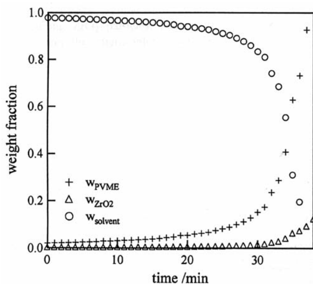
Fig. 2 Time variation of concentration of solvent, PVME, ZrO_2 accompanying with solvent evaporation estimated from weight loss measurement of a sample. The measurement was carried out for a sample with composition of 2.0 wt% PVME and 0.2 wt% ZrO_2
