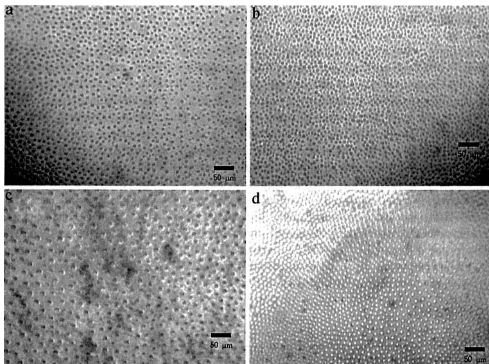
Fig. 6 Comparison of optical microscopy images of the self-assembling pattern for a 0 wt% ZrO 2 and 2.3 wt% PVME ( t=376 s), b 0 wt% ZrO 2 and 1.5 wt% PVME ( t=712 s), c 0.12 wt% ZrO 2 and 2.3 wt% PVME ( t=2076 s), d 0.12 wt% ZrO 2 and 2.0 wt PVME ( t=1638 s)
