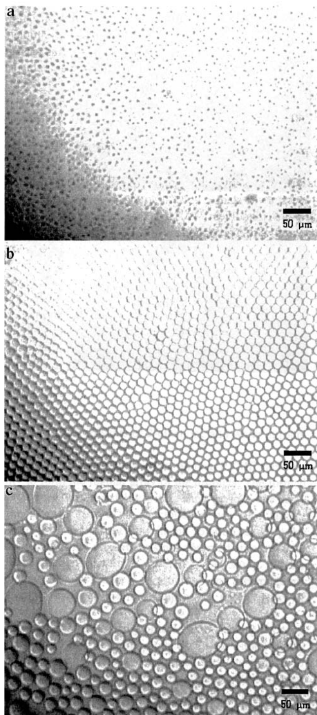
Fig. 5 Optical microscopy images of the self-assembling pattern for a polymer solution with a concentration of 2.3 wt% PVME (without adding ZrO_2 particles) at a 350, b 622, and c 856 s
